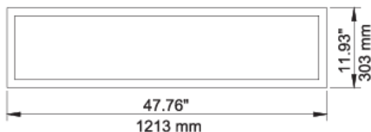
1x4 Front View
